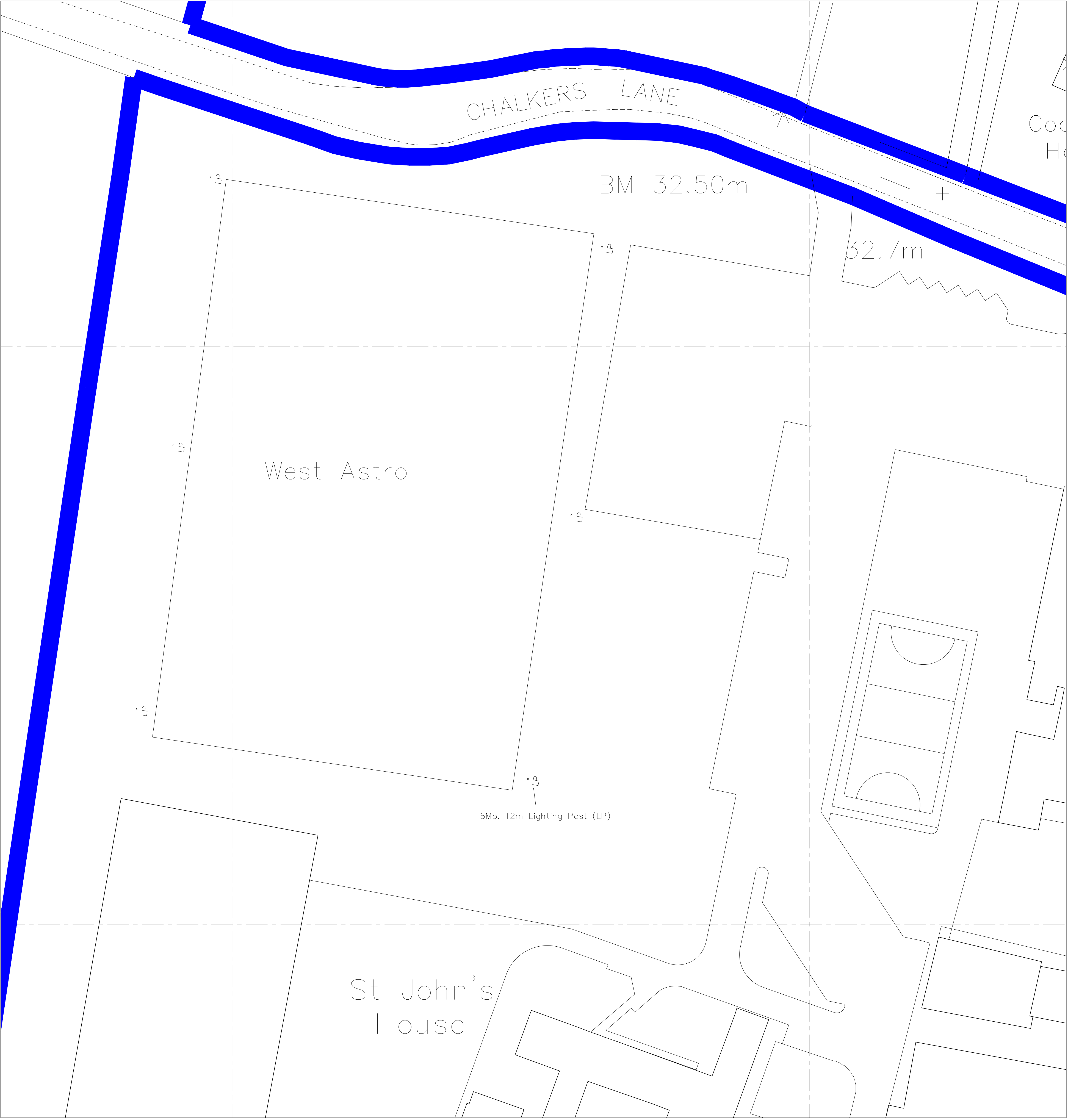
PROPOSED PLAN - Un Changed Scale 1:500
