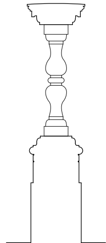
Existing Stone Balustade Standard Section Detail 1:20 @A1
