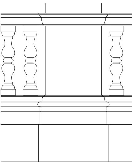
Existing Stone Balustade Standard Elevation Detail 1:25 @A1
