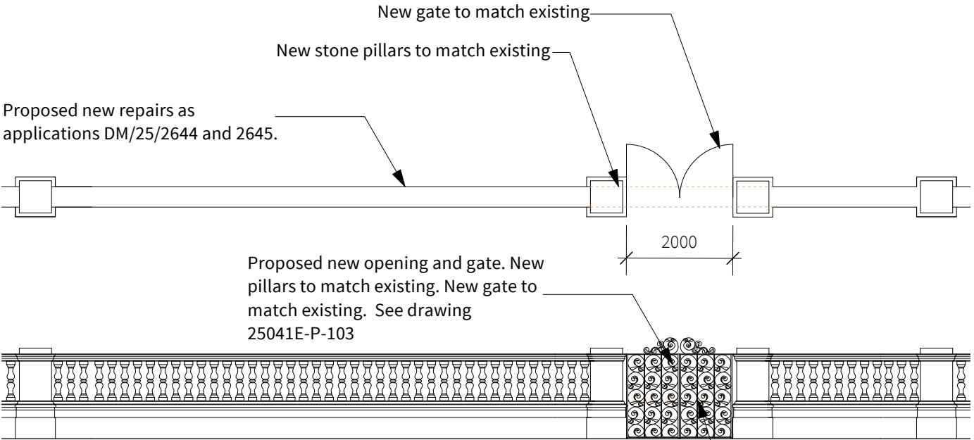
Lower section of wall to be cut away to create new opening
