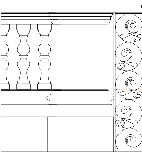
Proposed Stone Balustade - Standard Elevation Detail 1:25 @A1
