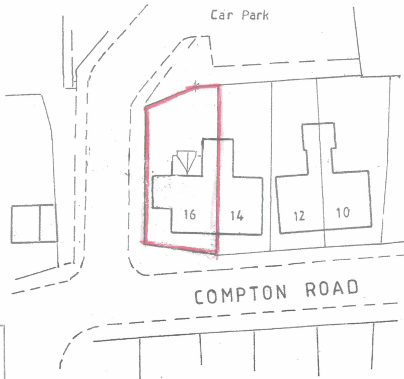
Block Plan 1:500
