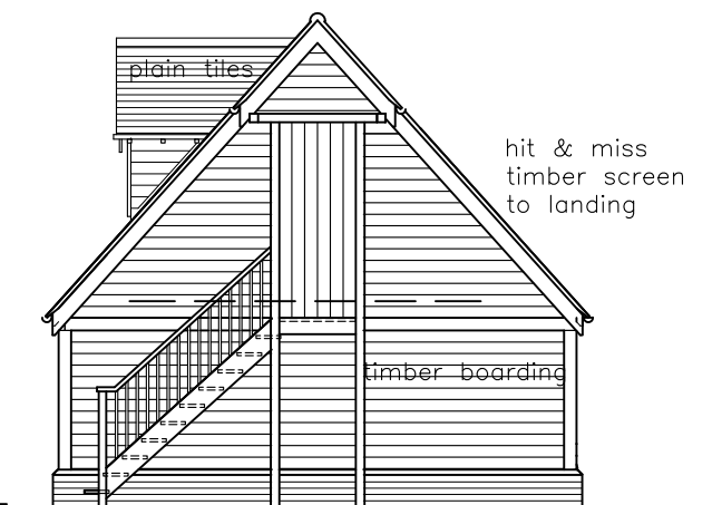
west elevation
