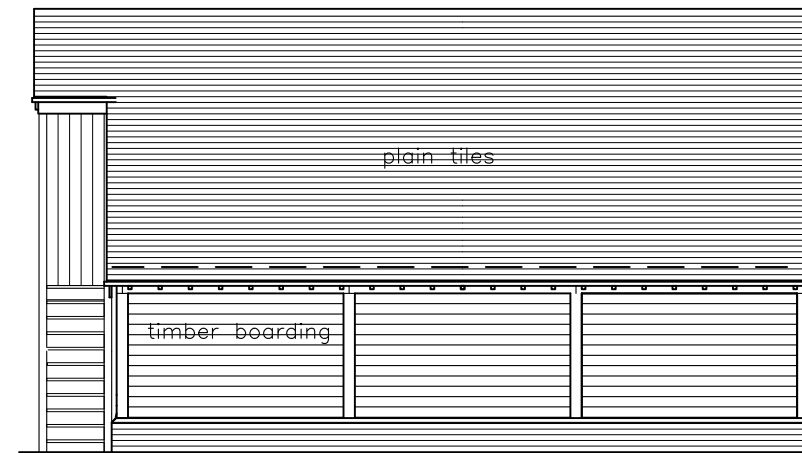
south elevation
