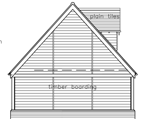
east elevation
