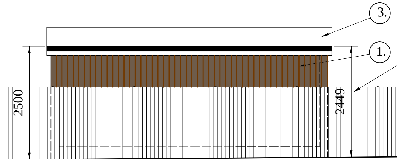
PROPOSED LEFT HAND SIDE ELEVATION
