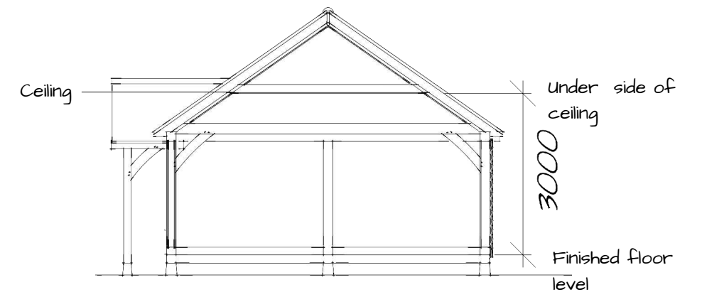
Proposed Cross-Section
