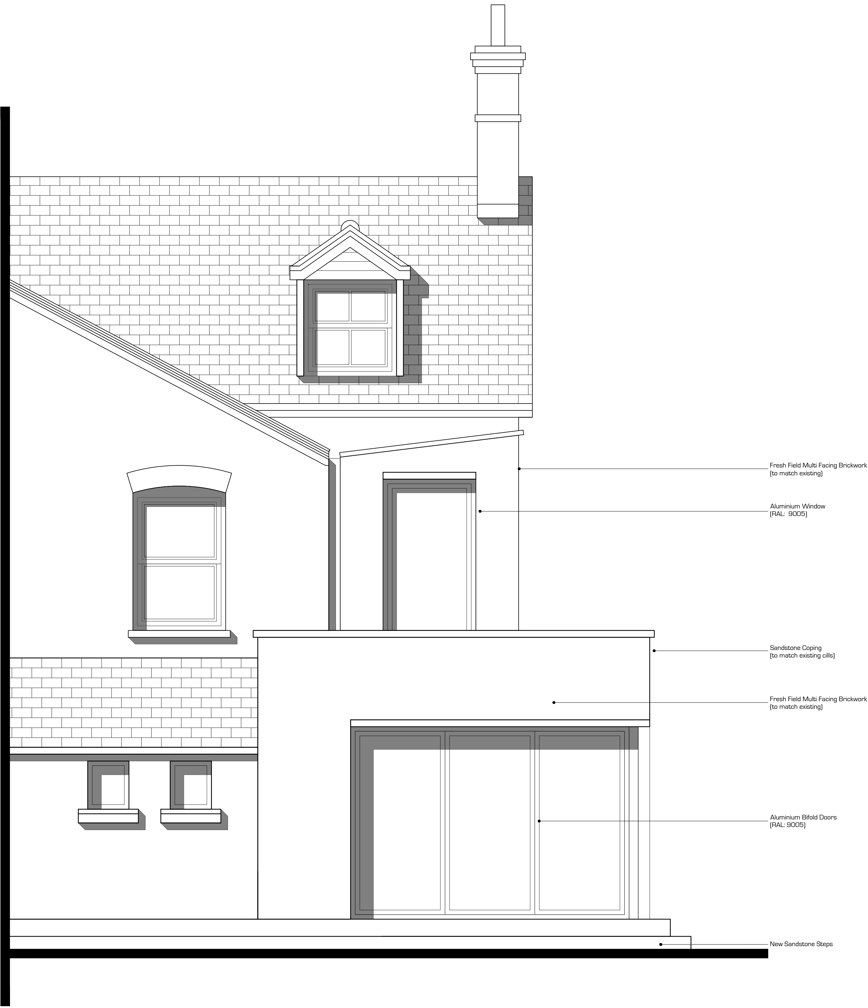
01 Proposed Rear Bay Study 1:25@A1
