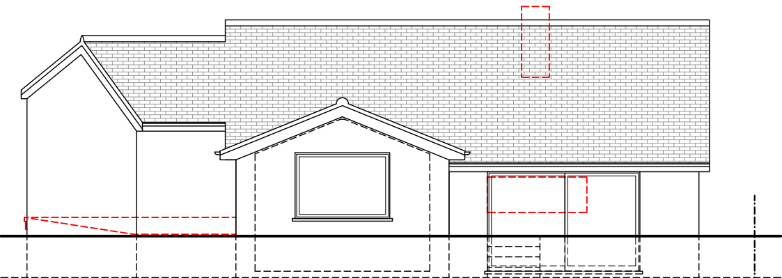
Proposed Rear Elevation (UGF Plan) Scale 1/100@A3
