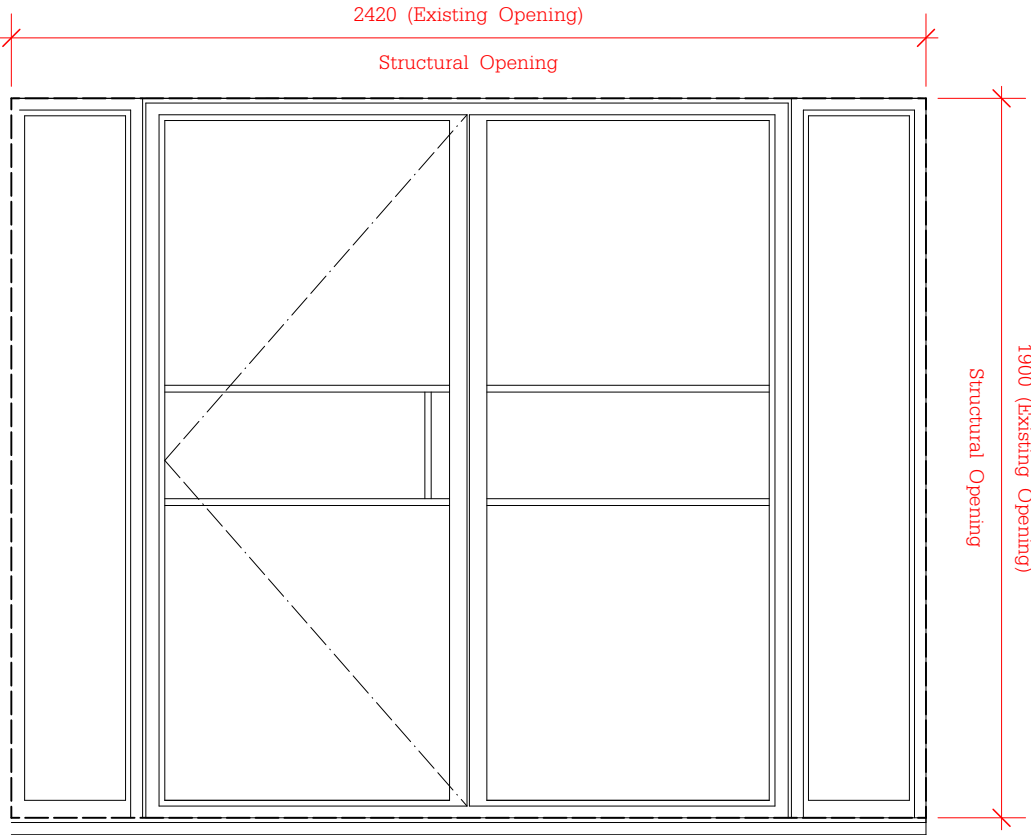
ED.005 Aluminium Crittal Style Door and Sidelights, set behind barn doors.
