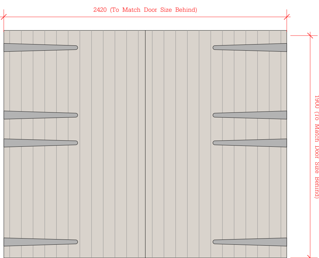
External Barn Doors 03 (for ED.004)
