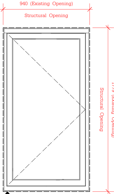
FFL to cill 210 ED.003 Painted timber outward opening door.
