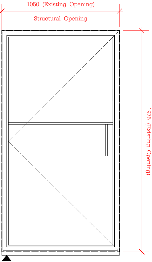
ED.001 Aluminium Crittal Style Door, set behind stable door.
