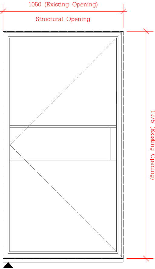
ED.002 Aluminium Crittal Style Door, set behind stable door.
