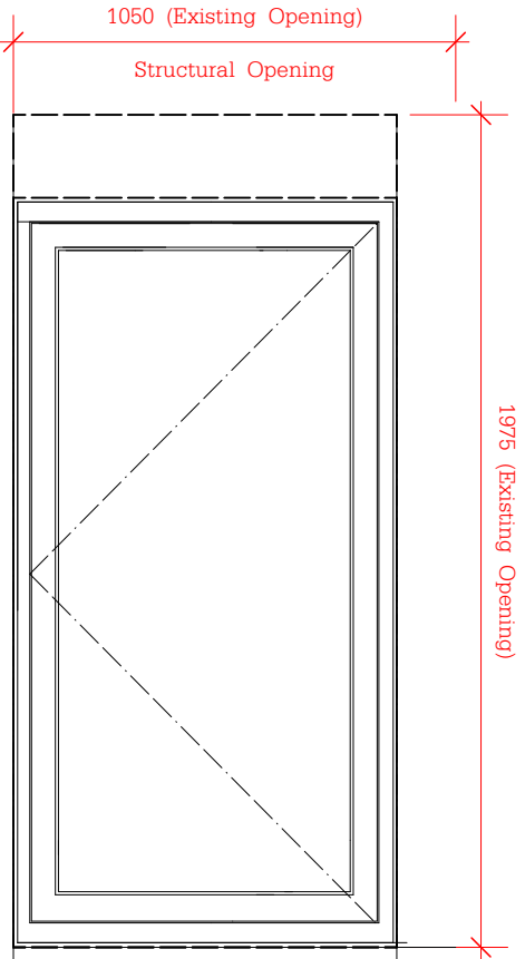
ED.004 Painted timber outward opening door
