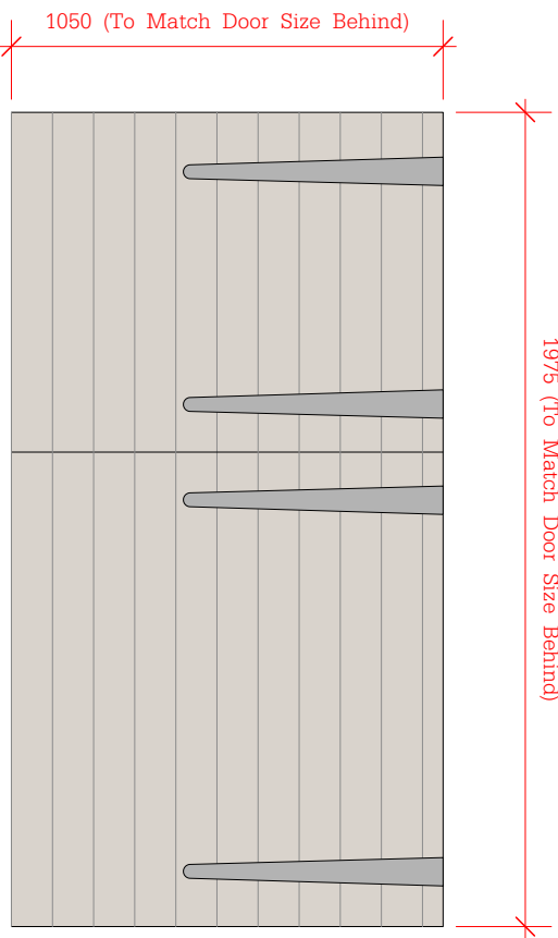
External Barn Doors 01 (for ED.001 and ED.002) Opening size to match door dimensions. Actual Opening size to be measured on site before creating.
