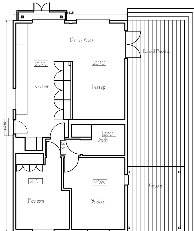
EXISTING FLOOR AYOIT
