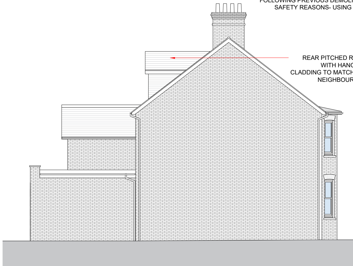
Side Elevation (N) 1:100
