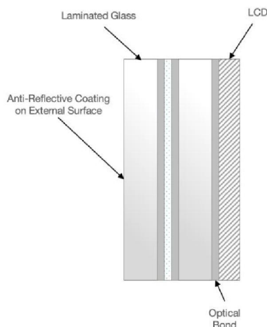
Figure 2 - composition cross section
