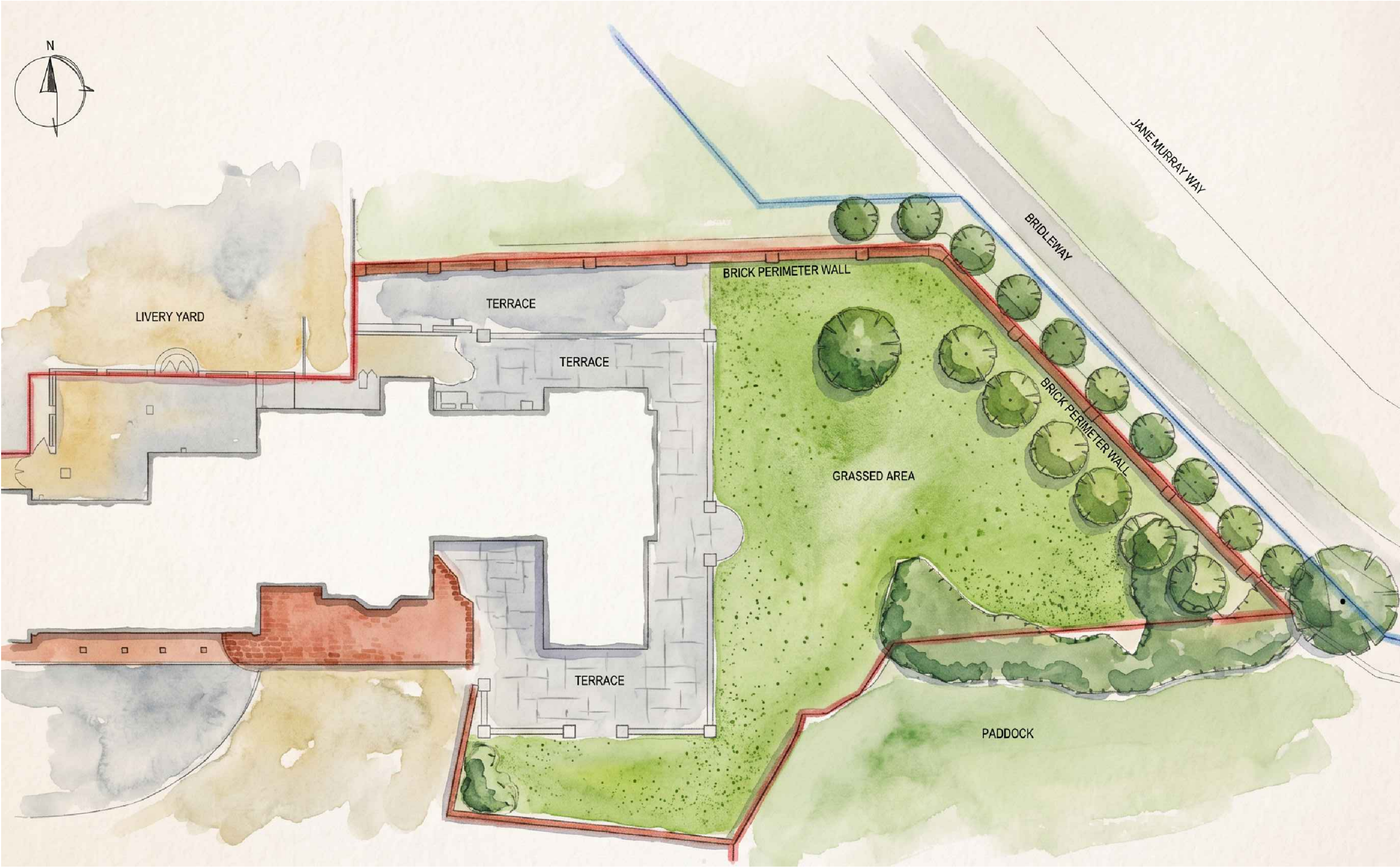
Landscape Treatment in Association with new Garden Wall - 1:100@A0
