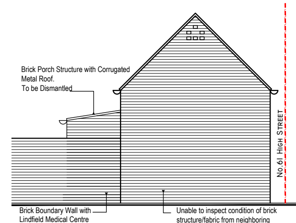
EXISTING WEST SIDE ELEVATION
