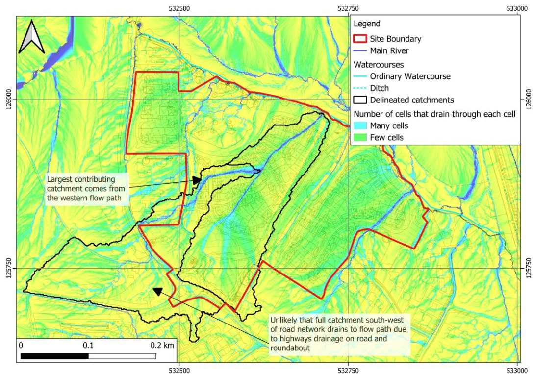
Figure 4-4 GIS analysis of surface water flow path
