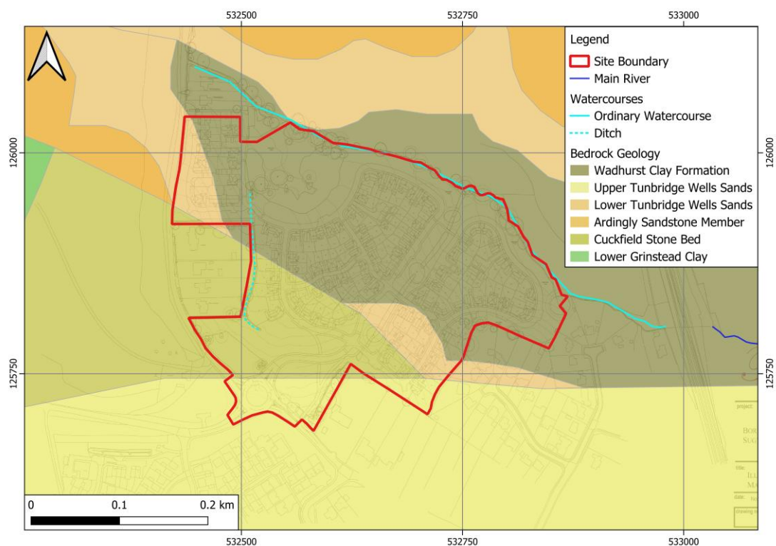
Figure 2-4 Bedrock Geology
