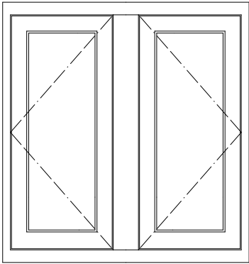
FFL to cill 694 EW.004 See Architects Specification for further details, finishes and performance requirements. New opening. To be measured on site before ordering.
