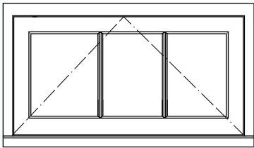
FFL to cill 1600 EW.001 See Architects Specification for further details, finishes and performance requirements. New opening. To be measured on site before ordering.
