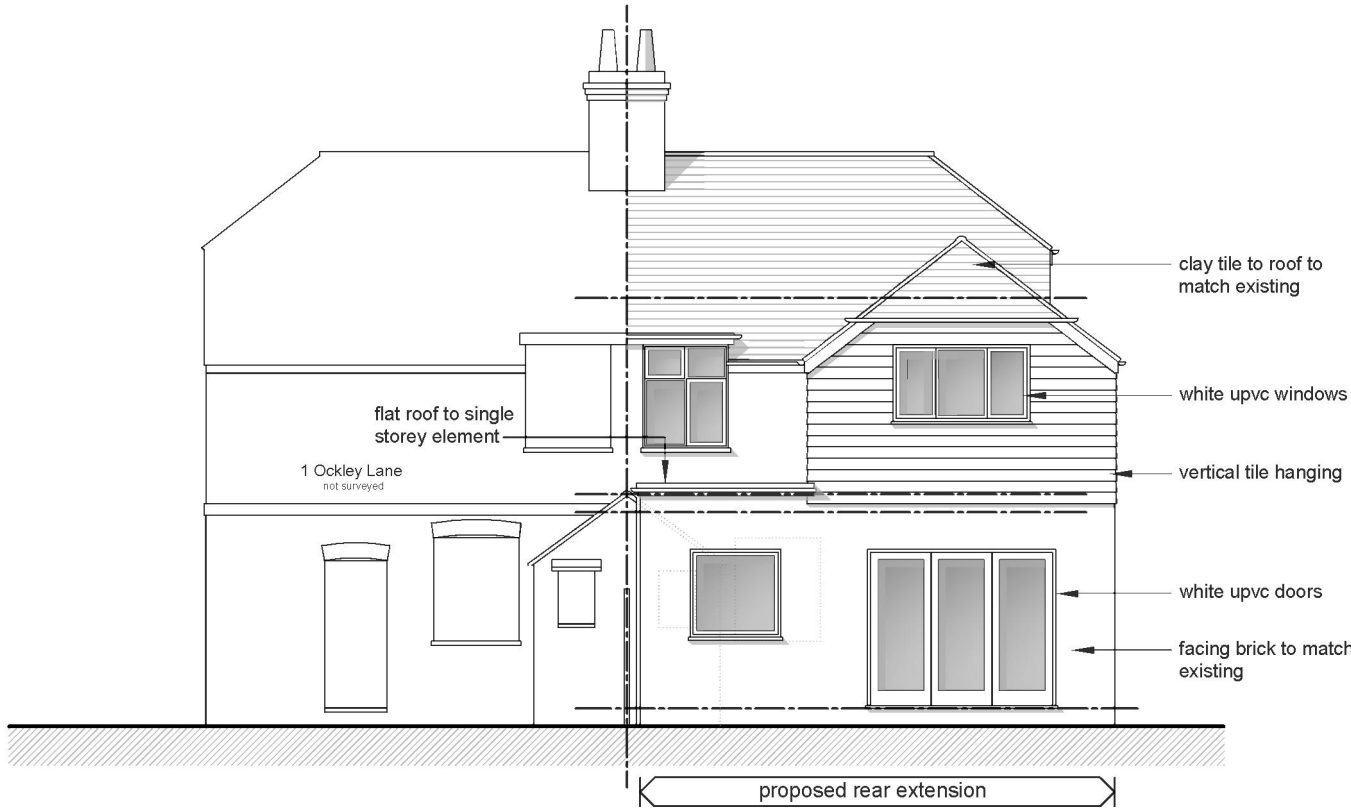
Rear Elevation
