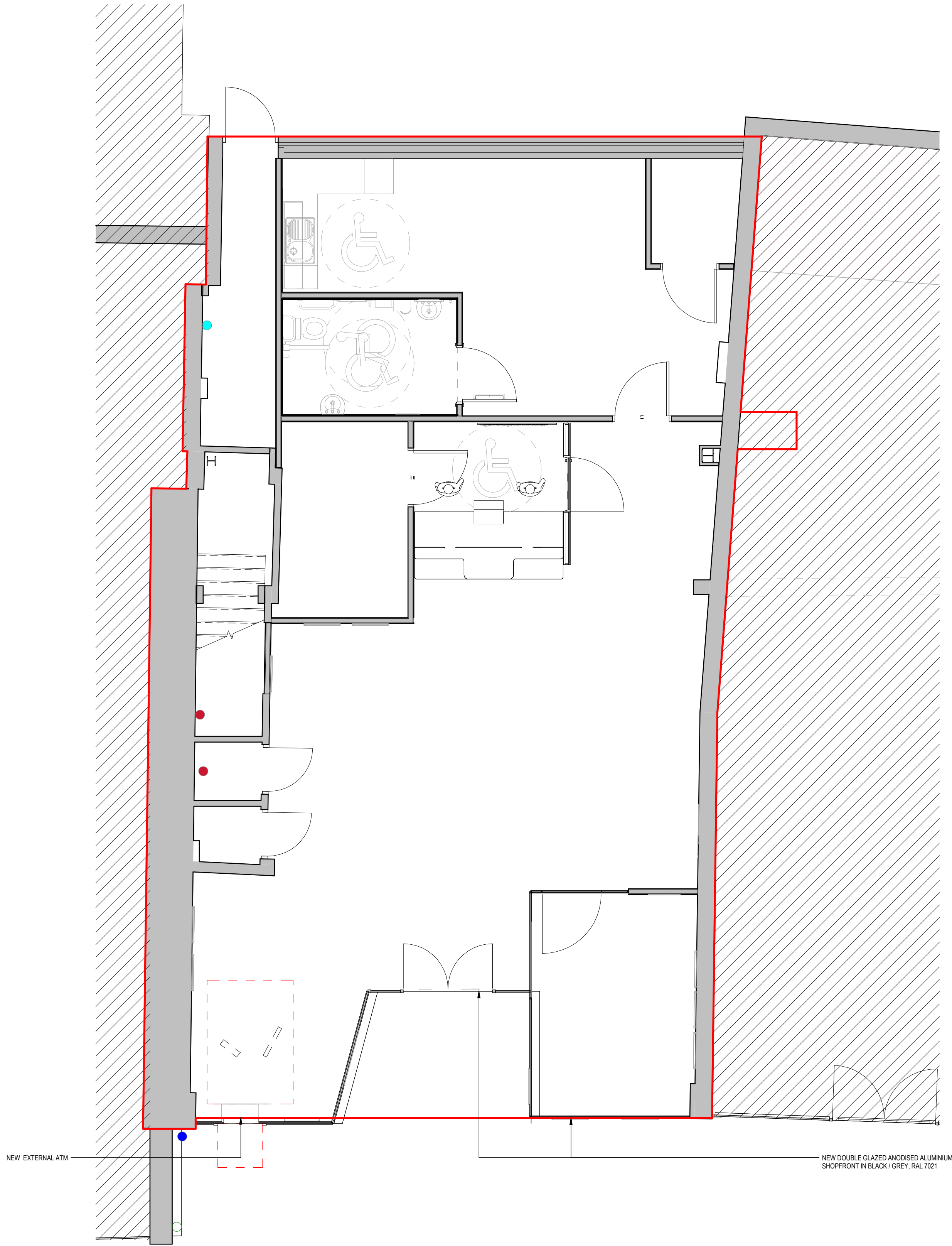
PROPOSED GA LAYOUT - PLANNING 1 : 50
