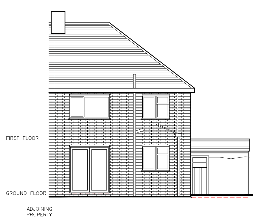
B) Existing Rear Elevation
