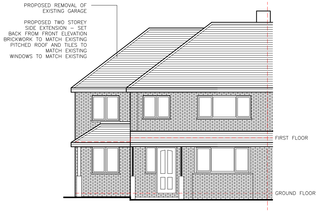
A) Proposed Front Elevation
