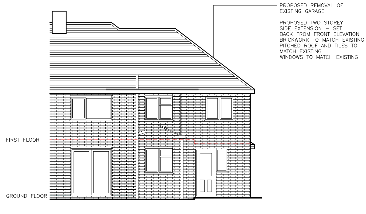
B) Proposed Rear Elevation
