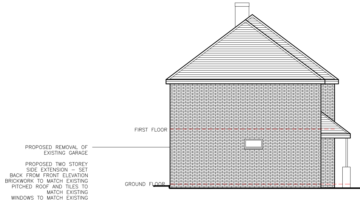
C) Proposed Side Elevation
