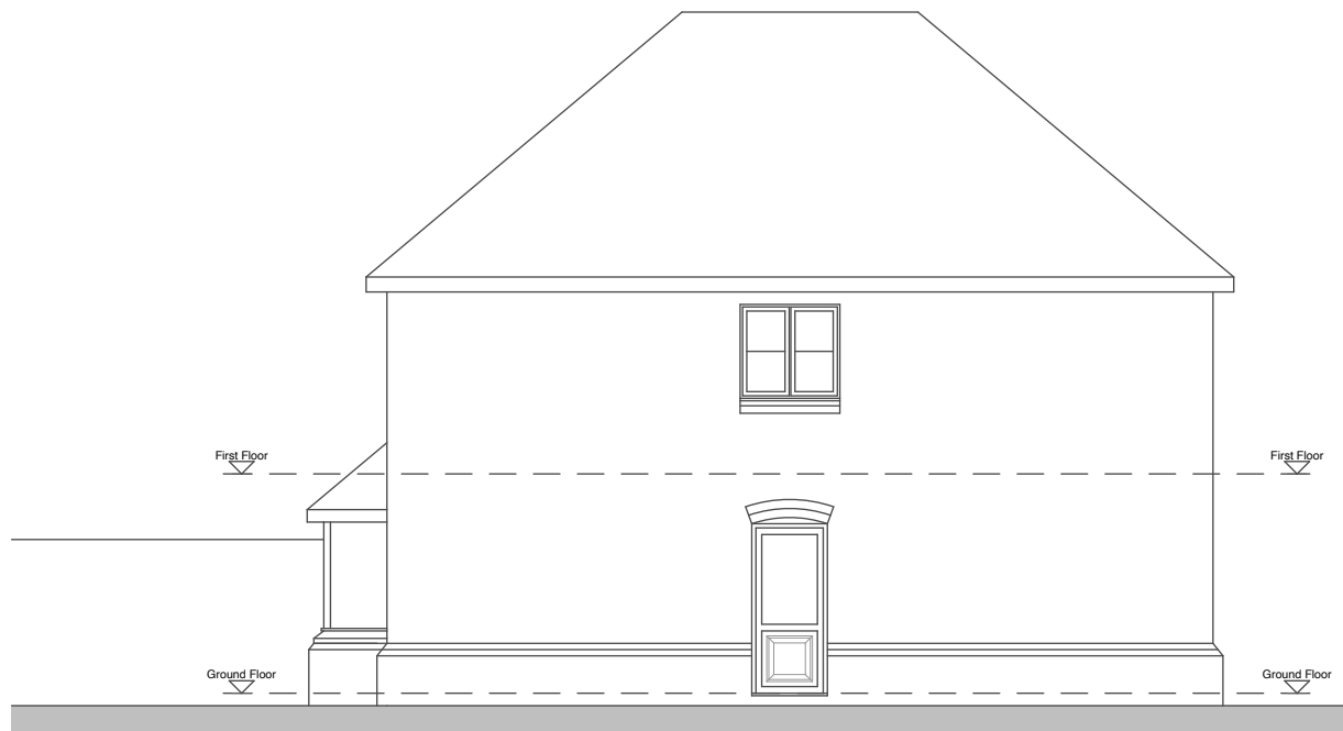
EAST ELEVATION 1:100
