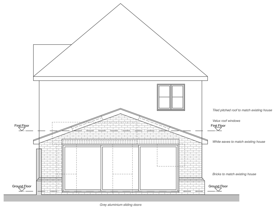
SOUTH ELEVATION 1:100
