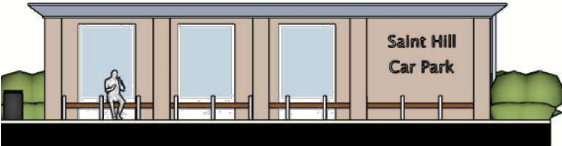
Proposed East Elevation 1:100
