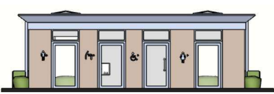
Proposed North Elevation 1:100
