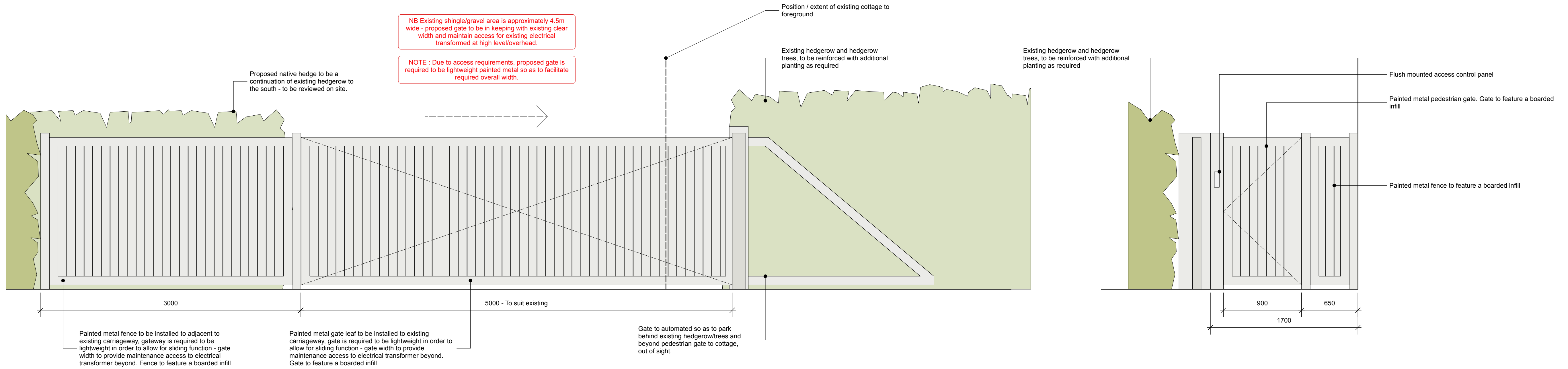
2 Proposed Rear Gate - Elevation Scale: 1:25
