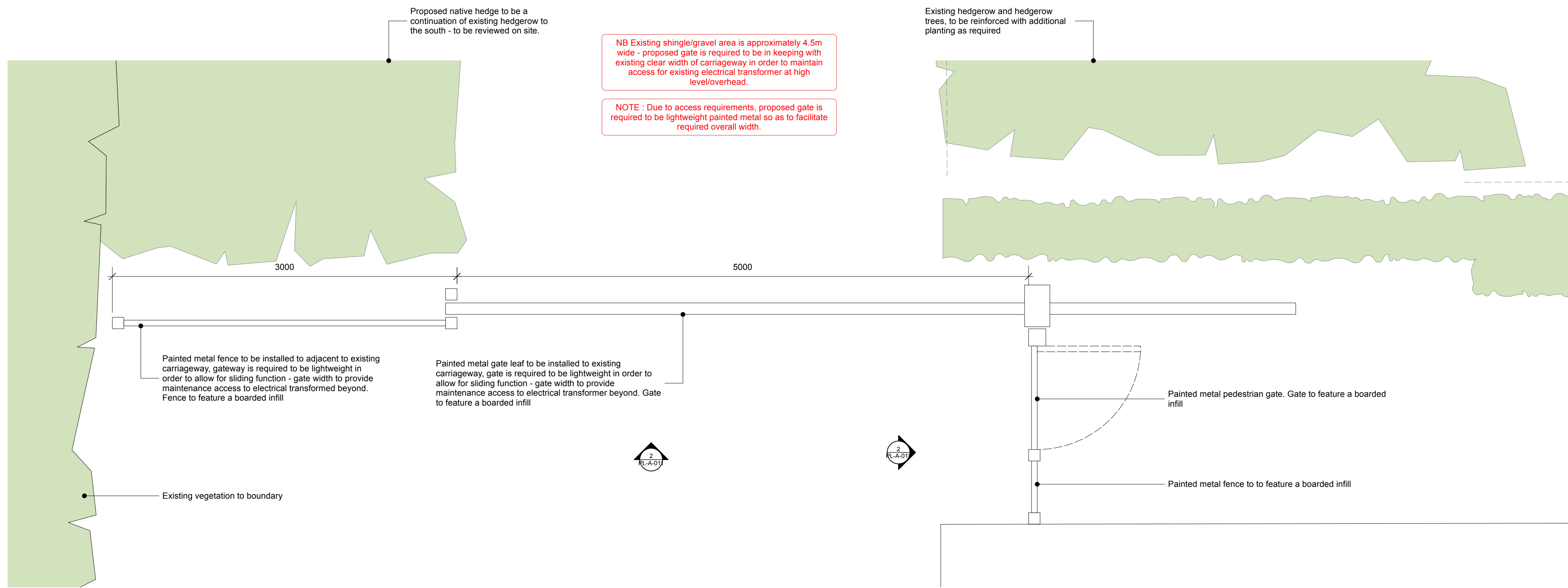
1 Proposed Rear Gate - Plan Scale: 1:25
