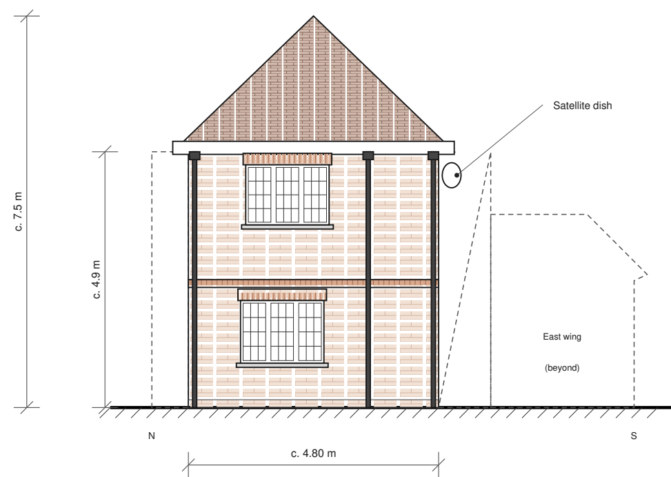
WEST ELEVATION (HIPPED END)
