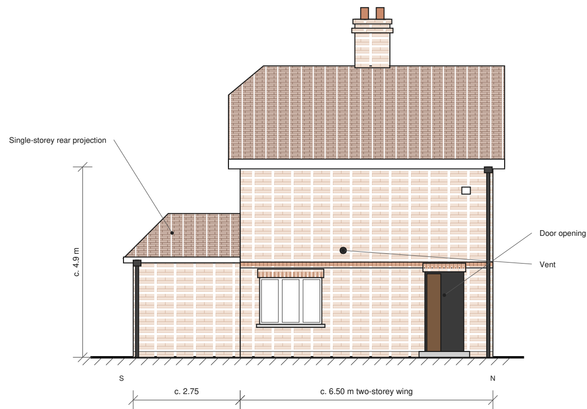
EAST ELEVATION (EAST WING)
