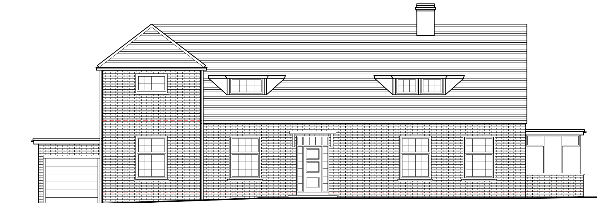
A) Existing Front Elevation
