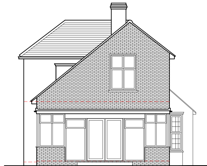
B) Existing Side Elevation
