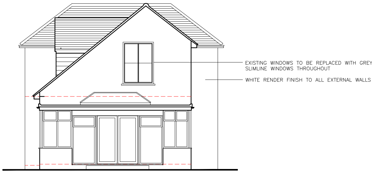
B) Proposed Side Elevation
