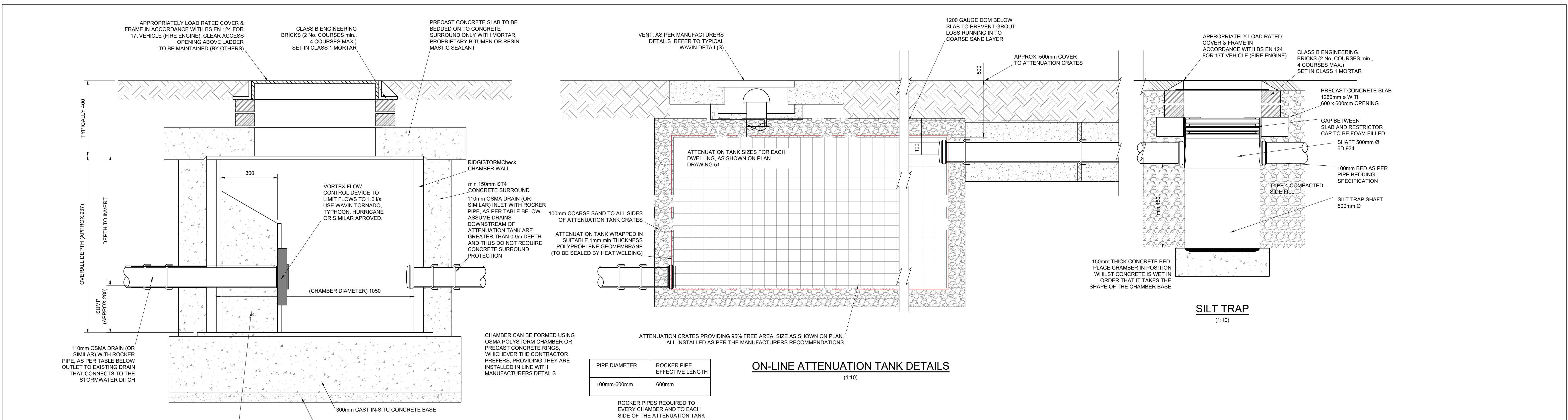
1.0 l/s RESTRICTED OUTFLOW CHAMBER (1:10)
