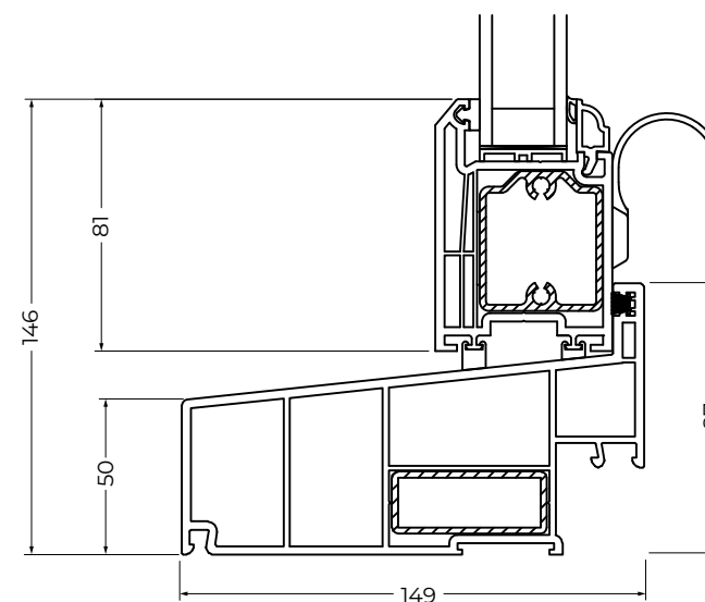
50mm deep flush cill
