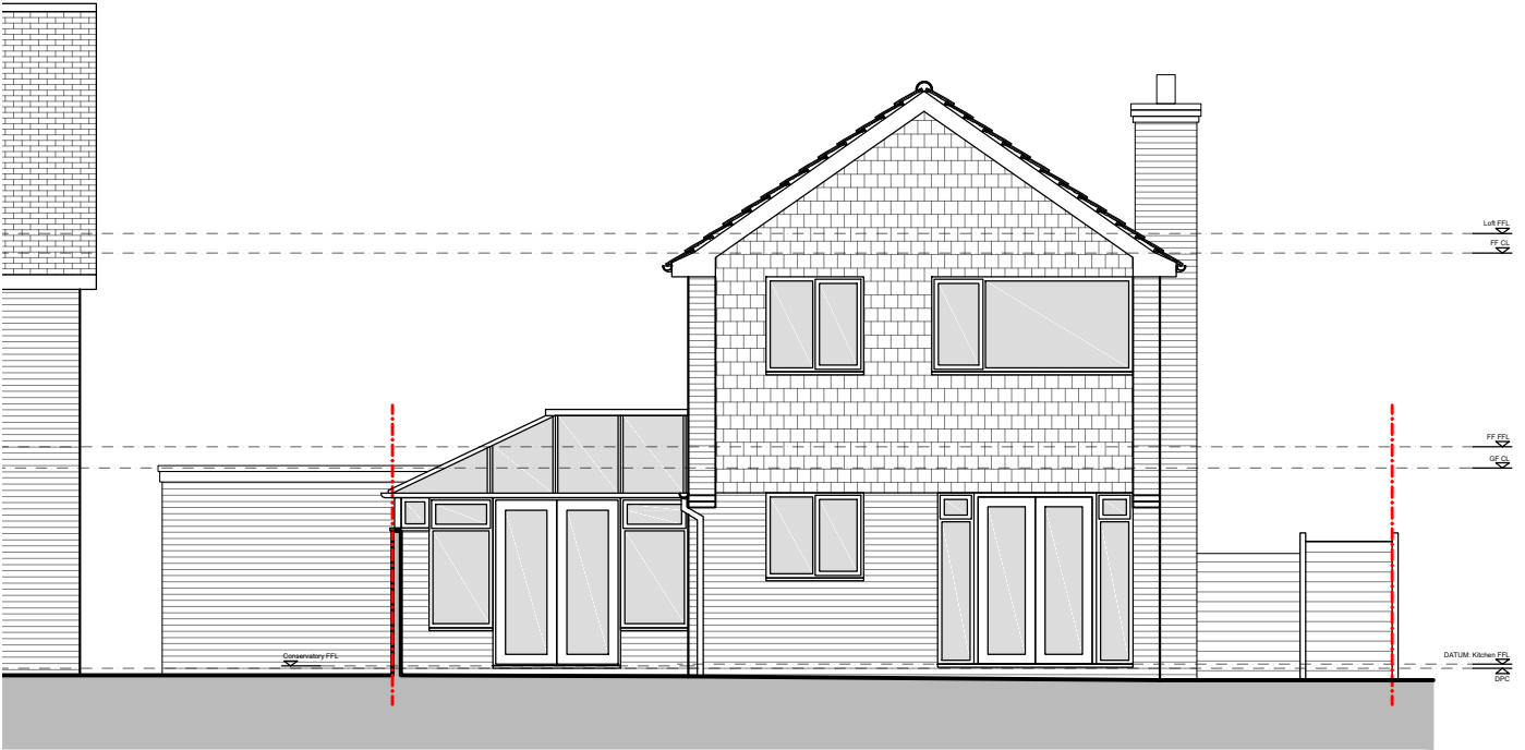
Rear (South) Elevation @ 1:100 Scale
