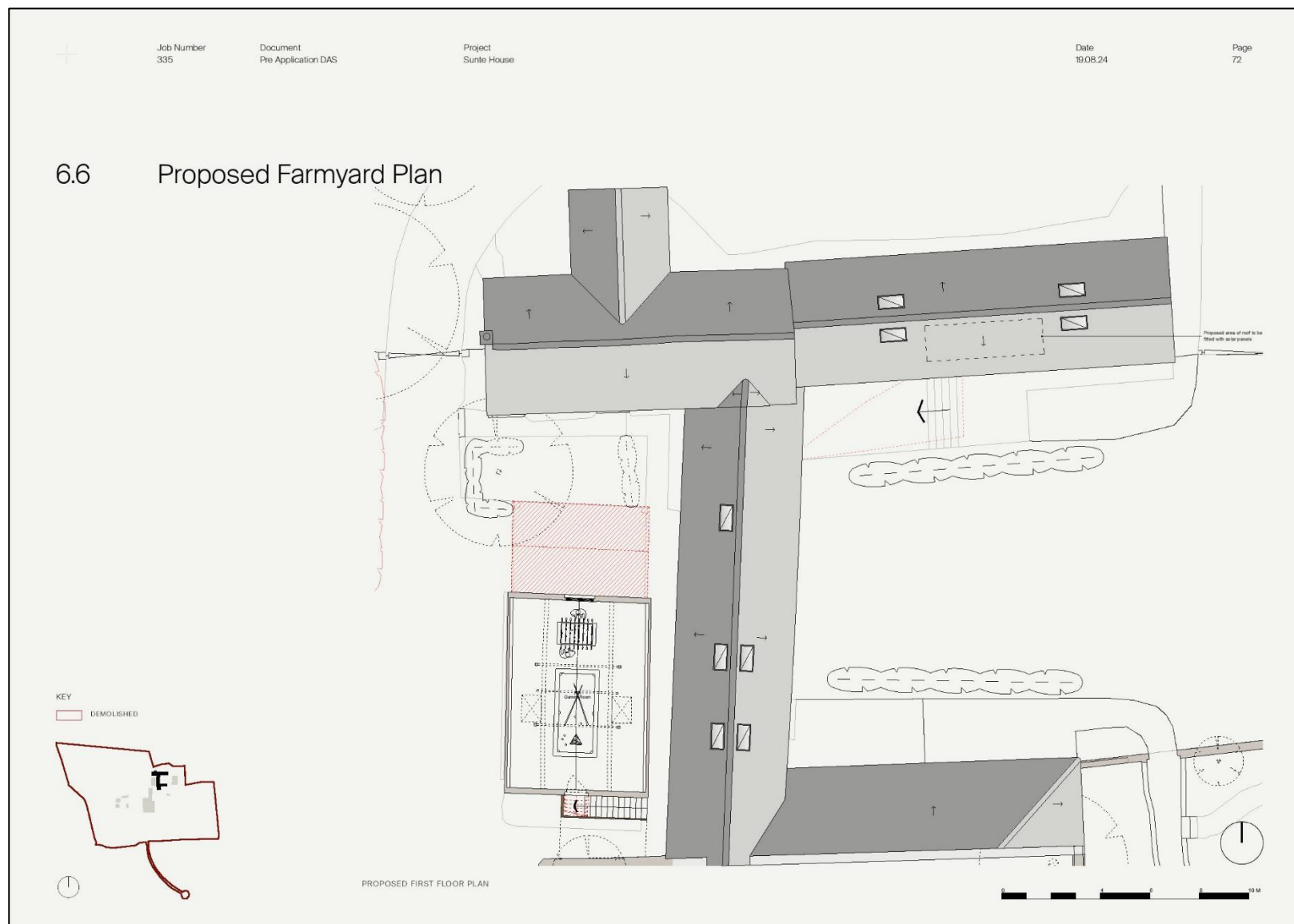
Figure 1.2: Proposed Farmyard Plan (B4, B5, B6, B7 and B8)
