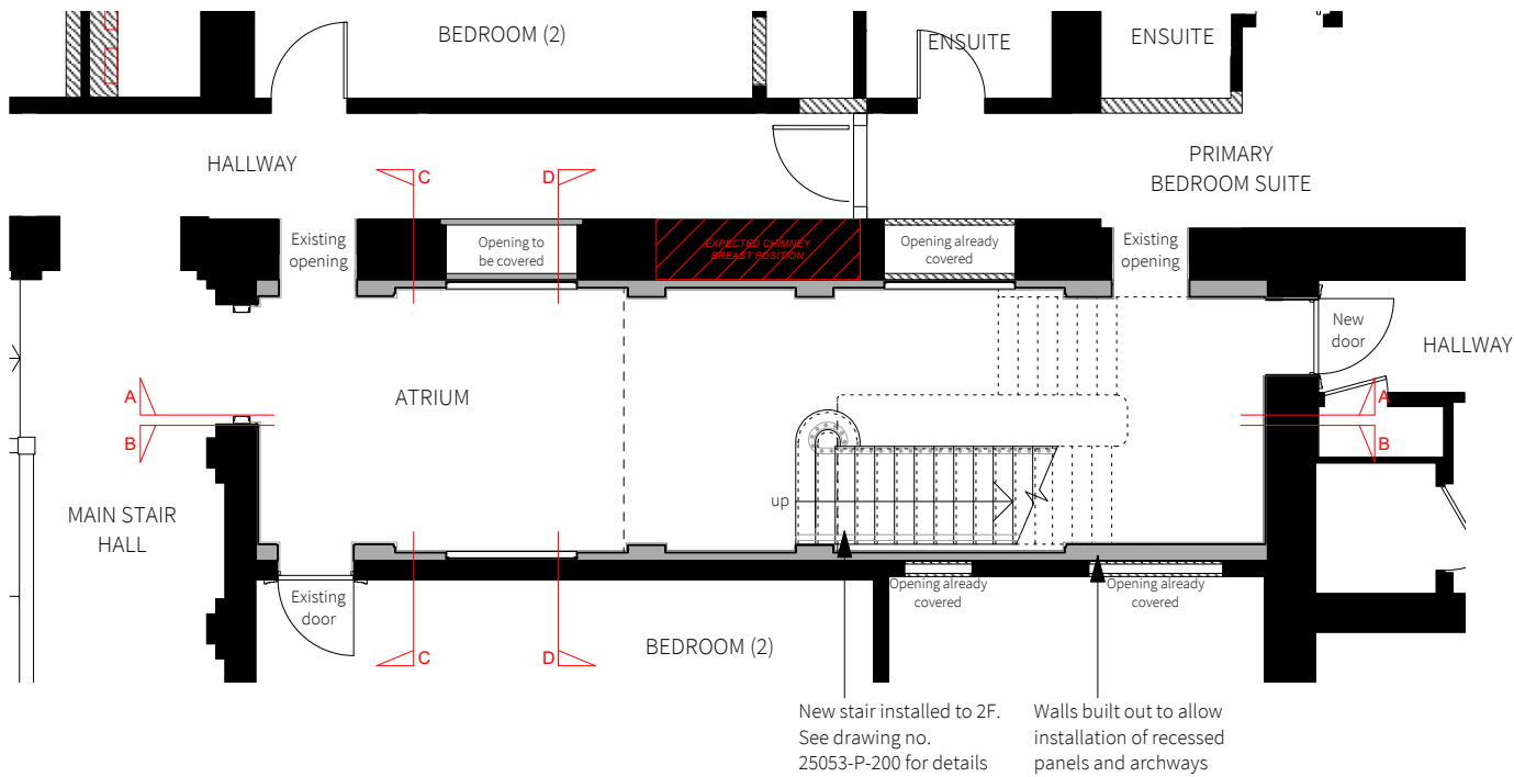
Proposed First Floor Plan Part plan showing atrium space. 1:100 @A3 / 1:50 @A1
