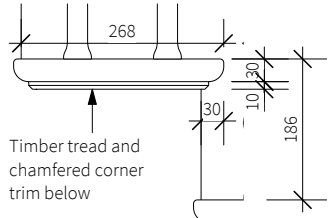
Handrail Wall Mount 1:10 @A3 / 1:5 @A1
