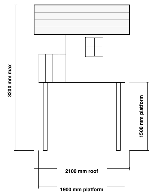
RIGHT SIDE ELEVATION
