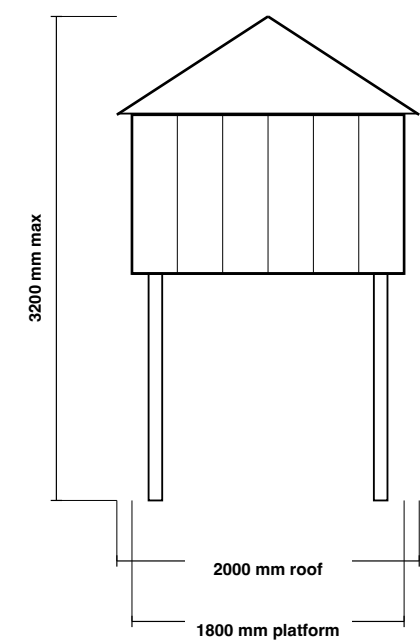
REAR ELEVATION
