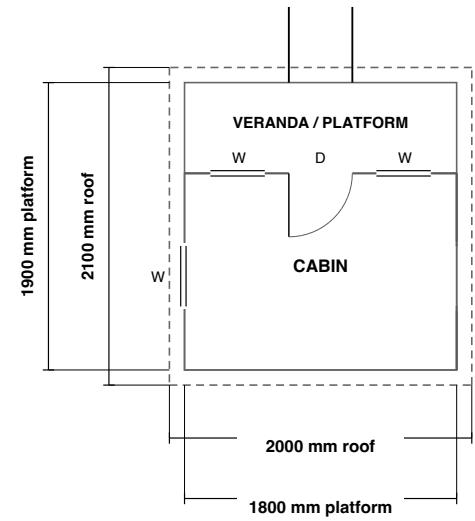
FLOOR / PLATFORM PLAN
