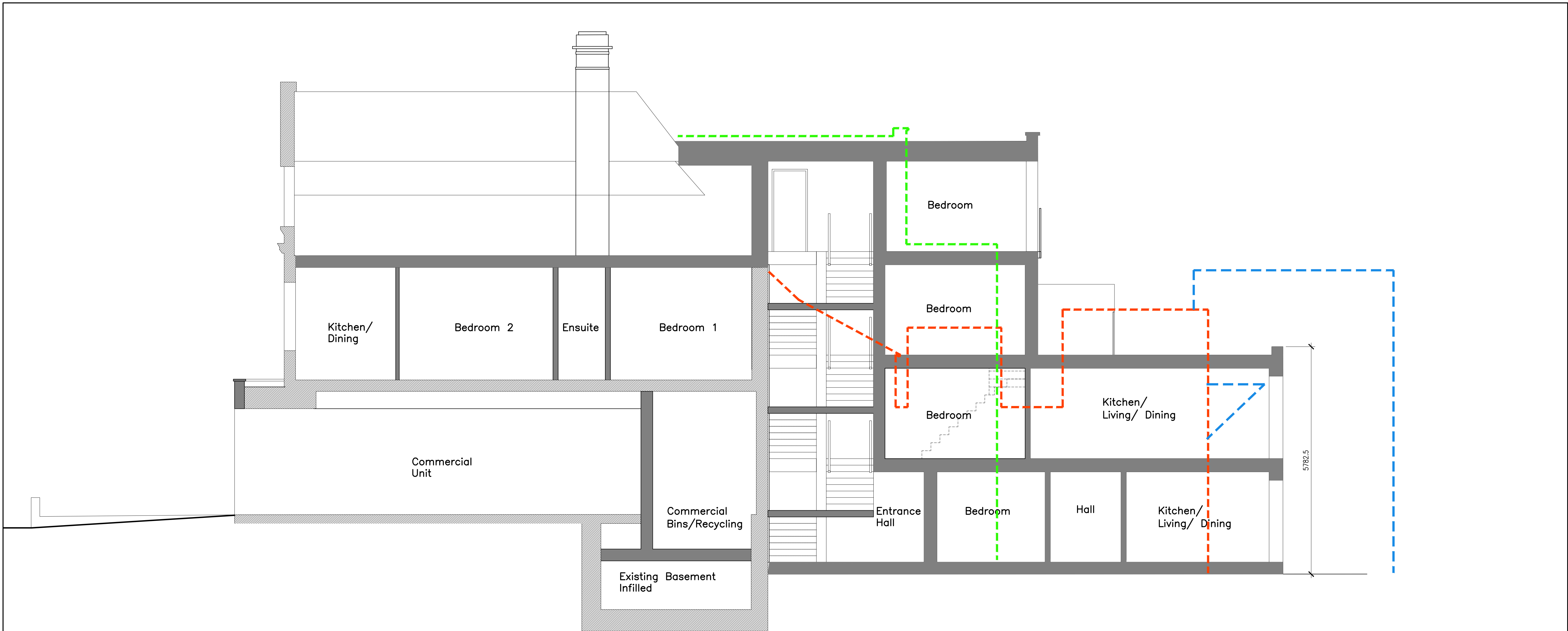
Section A-A 1:50 0 1 2 3 4 5 6 7 8 9 10 Scale In Metres
