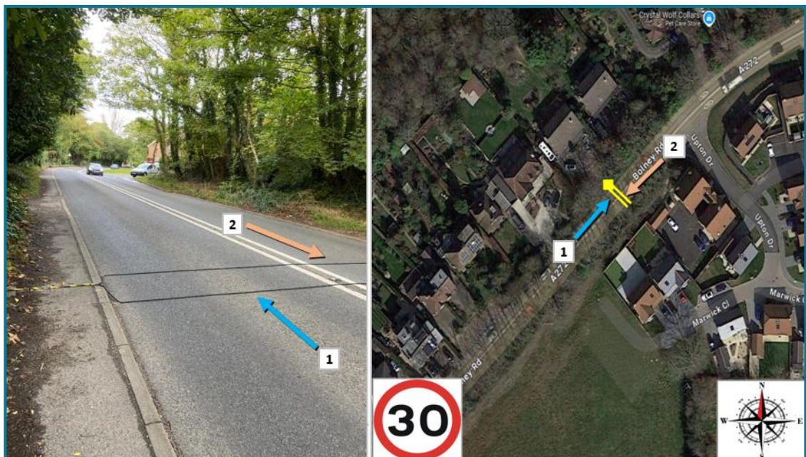
Figure 2.6 – Location of Automatic Traffic Count on Bolney Road (A272) fronting the site
