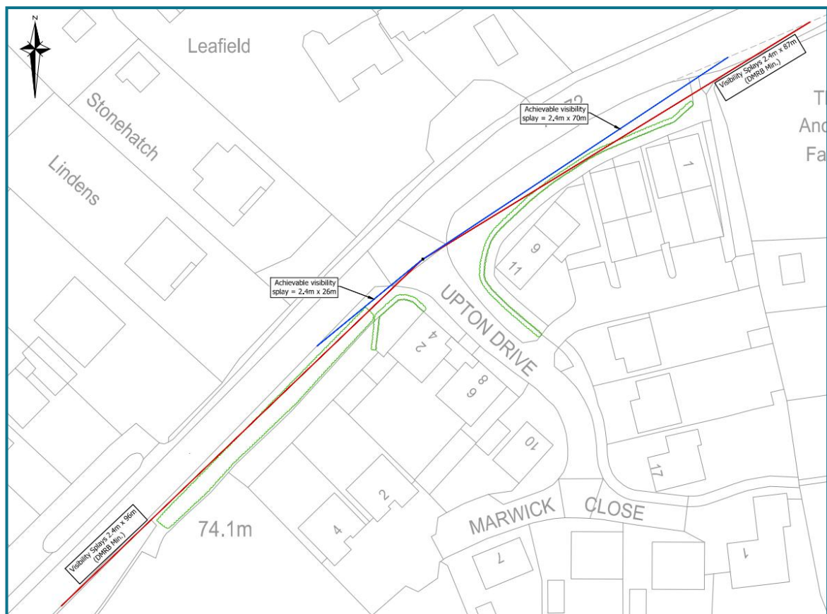
Figure 2.7 – Visibility splays achievable from Upton Drive / A272 access point
