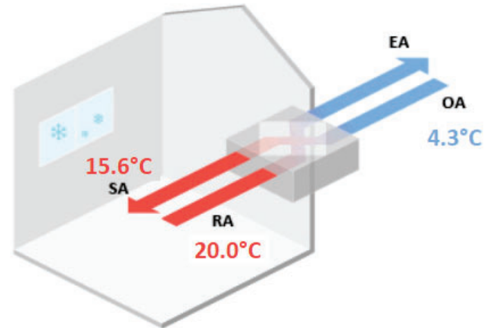
Lossnay Unit
