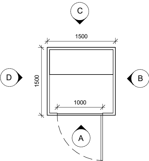
PLAN VIEW 1:50
