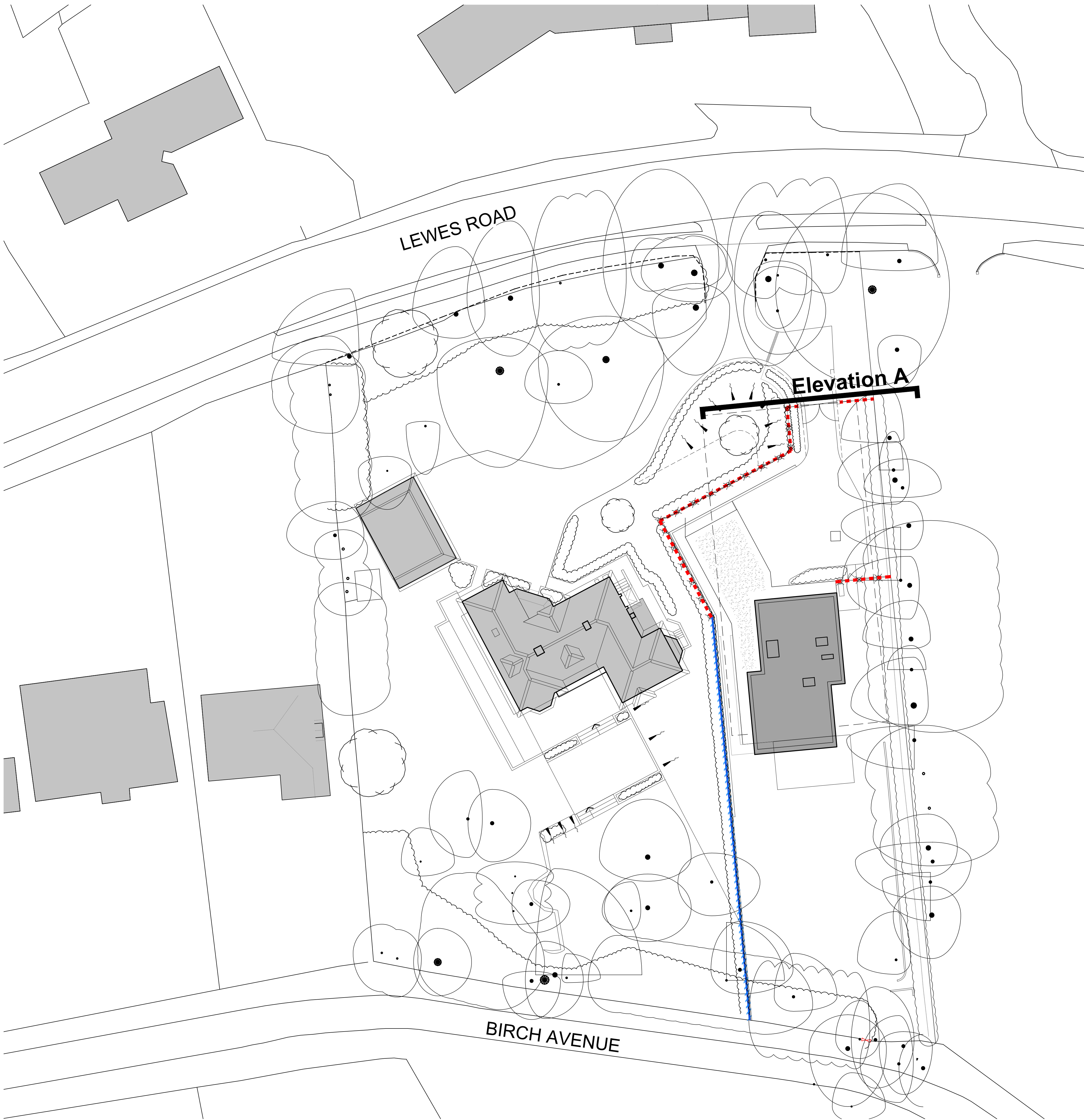
Proposed Boundary Treatments Plan 1:50 scale
