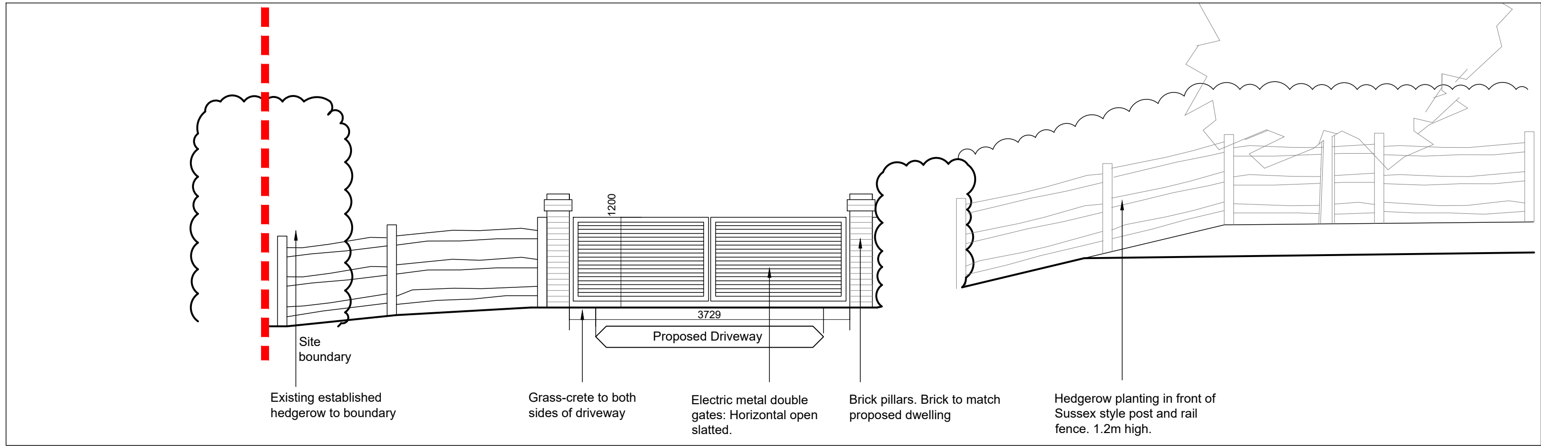
Proposed Elevation A 1:50 scale
