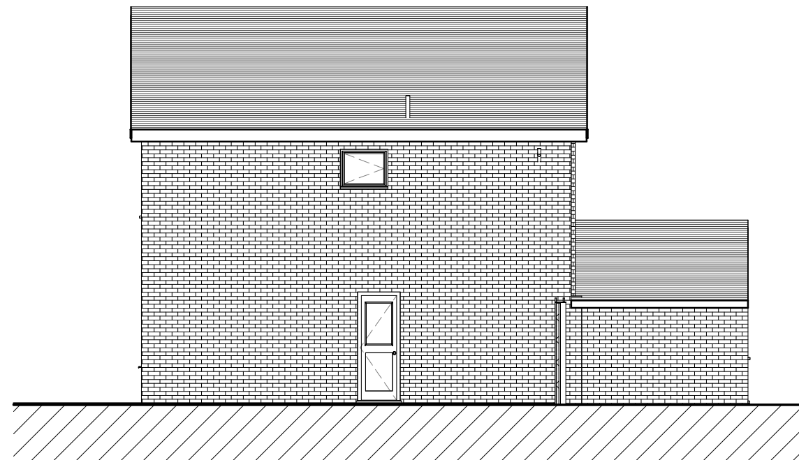
Proposed Side Elevation II. 1 : 100
