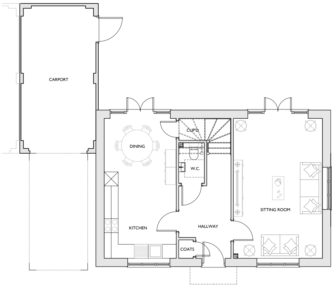
GROUND FLOOR PLAN 1,282 sqft PLOT 27
