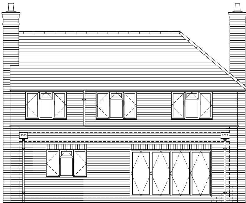
Rear Elevation (West Facing) (Scale 1:100)
