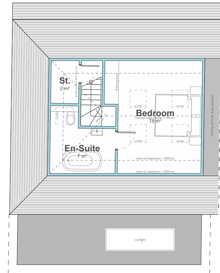
Proposed Loft Plan Scale 1:100 @ A3
