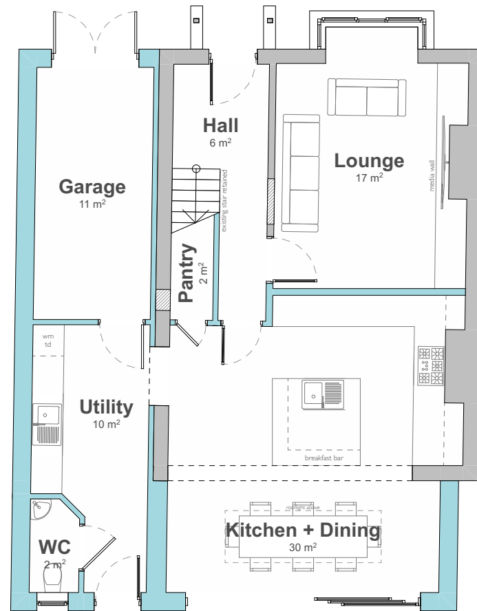
Proposed Ground Floor Plan Scale 1:100 @ A3
