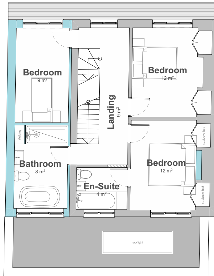
Proposed First Floor Plan Scale 1:100 @ A3
