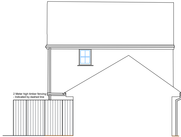
REAR ELEVATION
