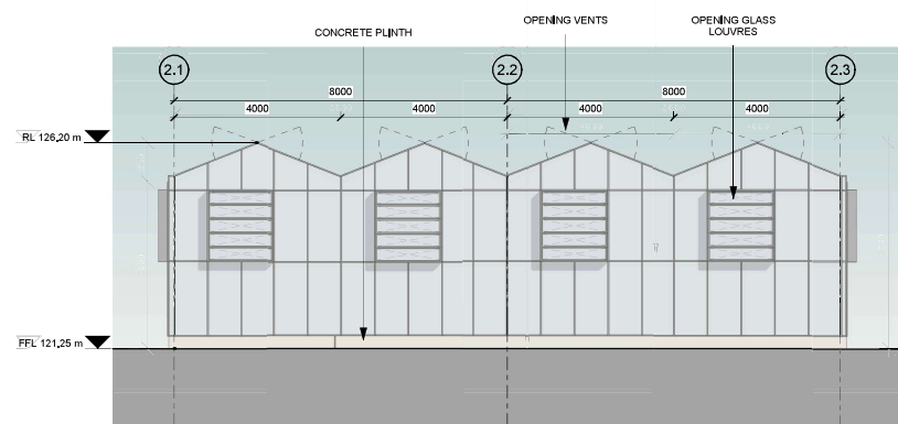
5 Proposed Elevation GH2 - West 1:100
