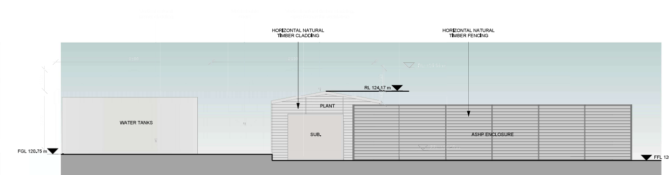
11 Proposed Elevation Plant - North 1:100
