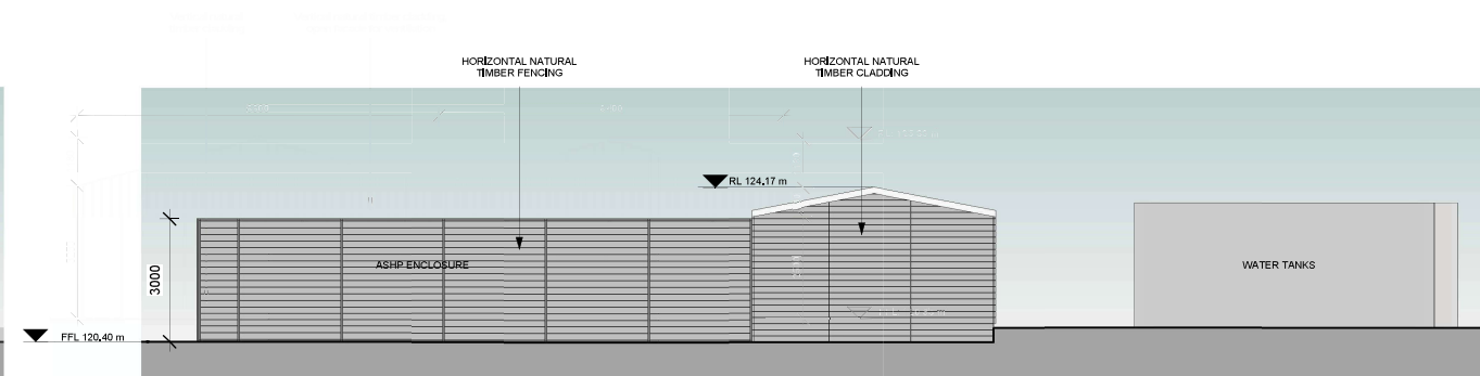
10 Proposed Elevation Plant - South 1:100
