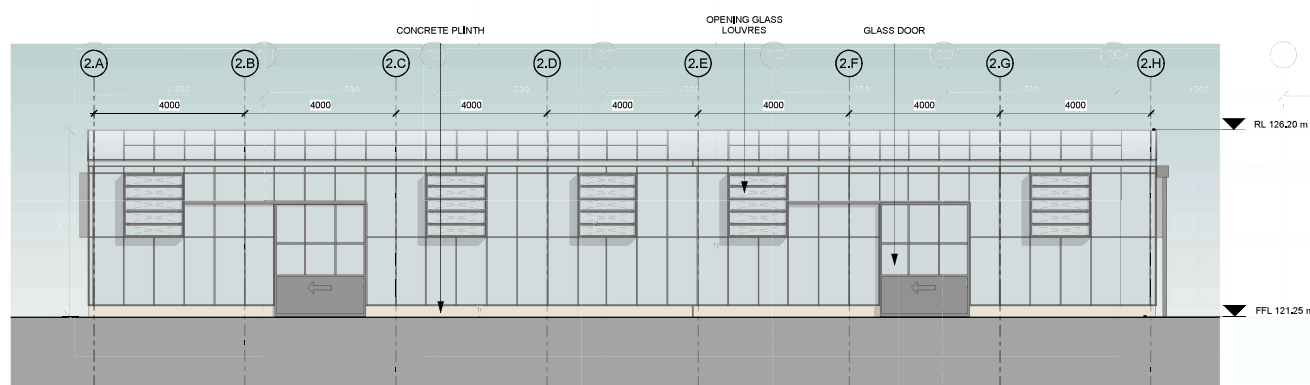
6 Proposed Elevation GH2 - South 1:100
