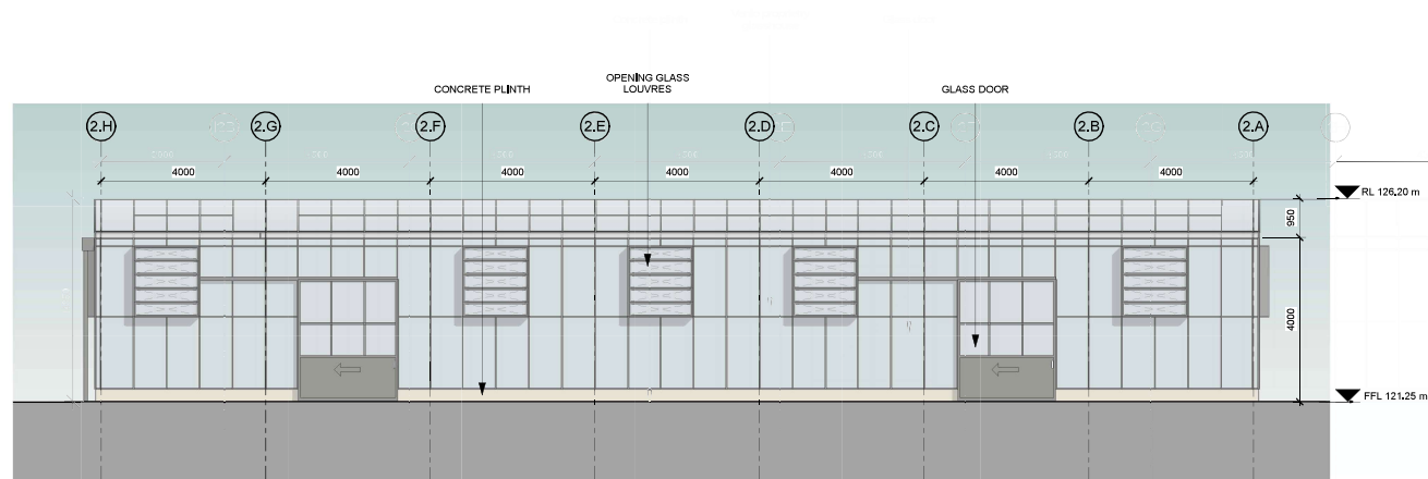
7 Proposed Elevation GH2 - North 1:100
