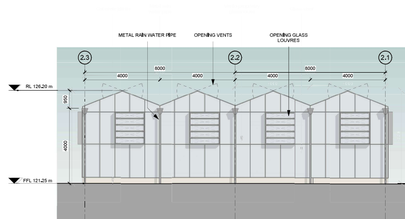
8 Proposed Elevation GH2 - East 1:100
