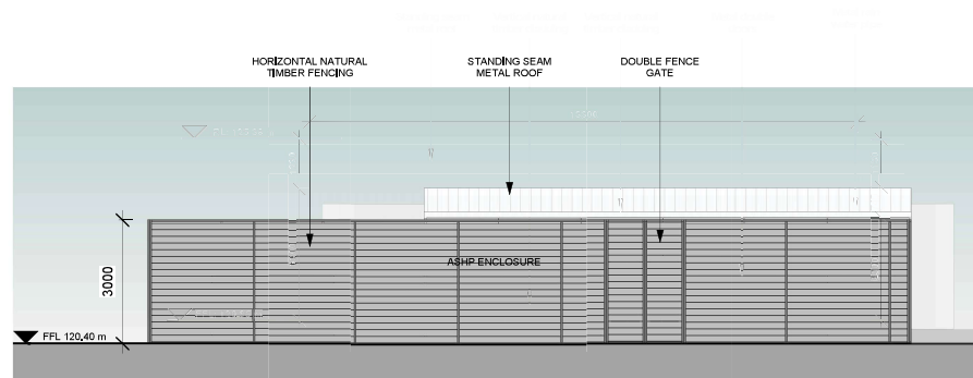
9 Proposed Elevation Plant - West 1:100
