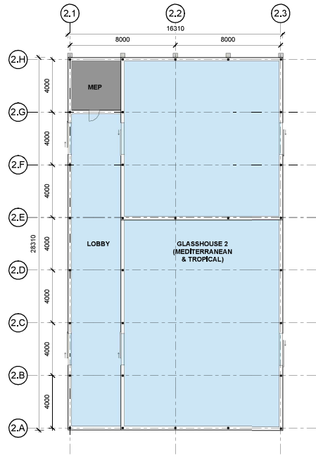
2 Glasshouse 2 - Ground floor plan 1:200
