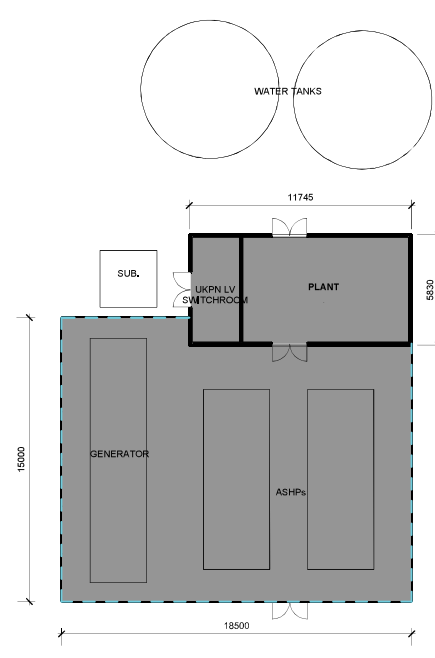
4 Plant - Ground floor plan 1:200
