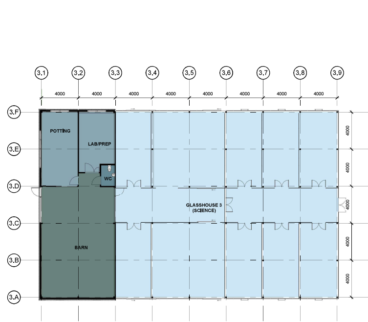
1 Glasshouse 3 - Ground floor plan 1:200
