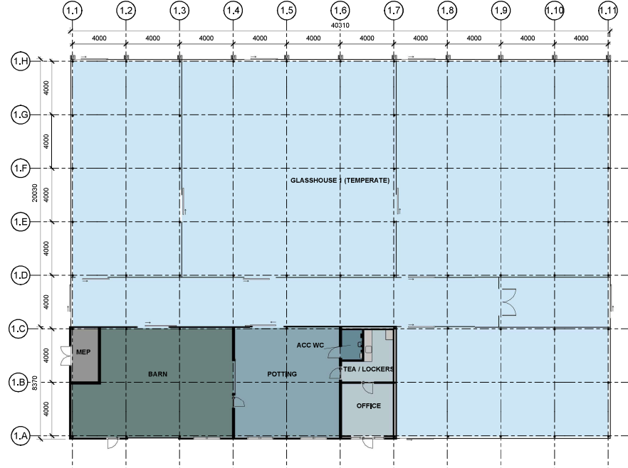
3 Glasshouse 1 - Ground floor plan 1:200
