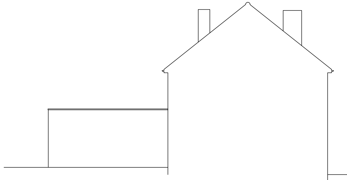
04 Side Elevation - As Existing 2001 1:100 (at A3)
