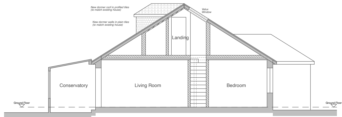
SOUTH SECTION/ELEVATION 1:100
