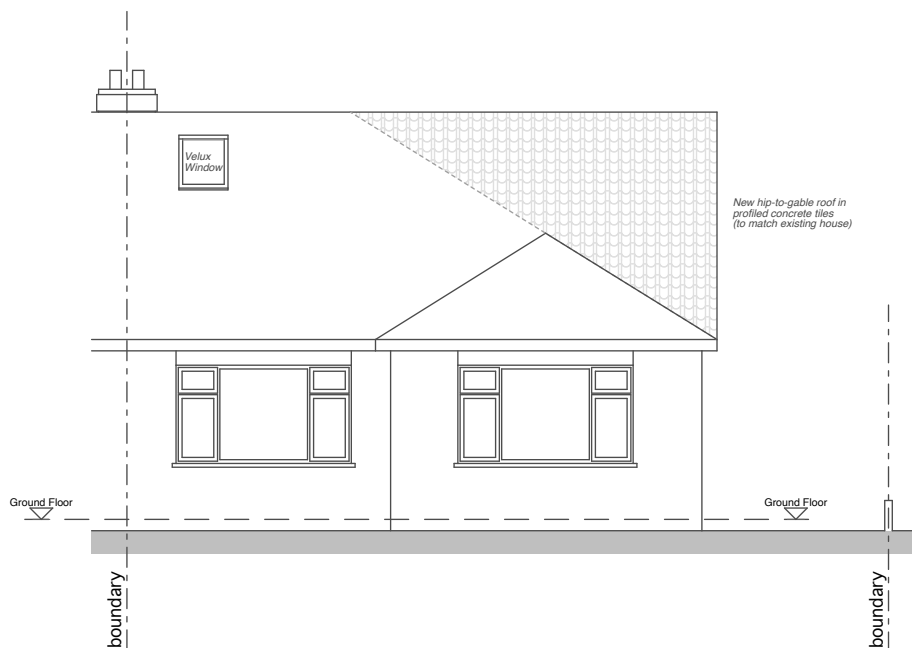
EAST ELEVATION 1:100
