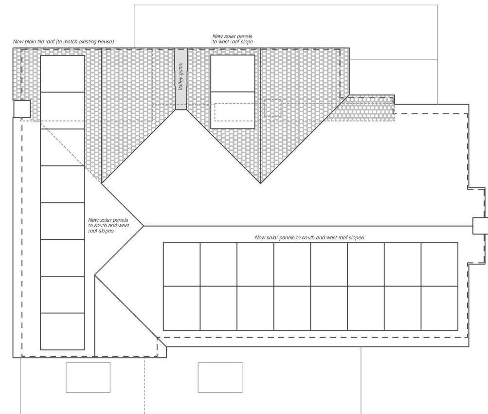
ROOF PLAN 1:100
